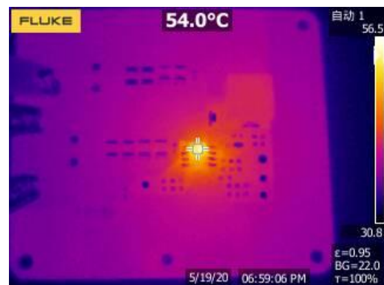
Figure 25. Thermal, 3.3Vout/2A
