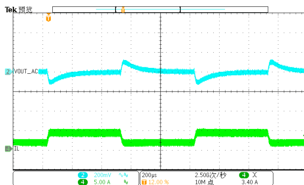
Figure 20. Load Transient (1.25A-3.75A, 1.6A/us)
