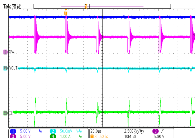
Figure 18. Output Ripple (Iload=0A, USM)
