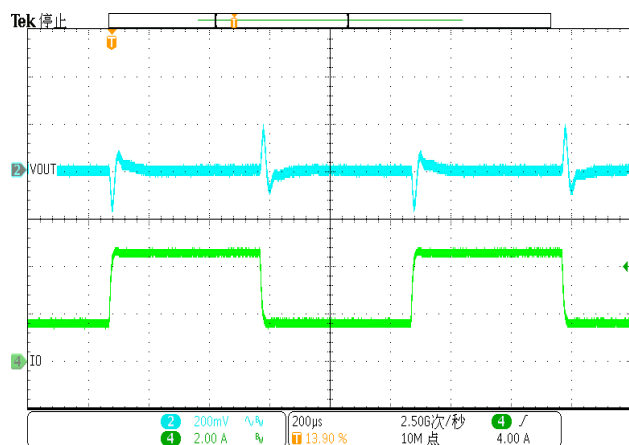
Figure 16. Load Transient (1.5A-4.5A, 1.6A/us)
