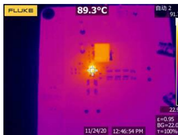
Figure 21. Thermal, 12VIN, 5Vout, 6A
