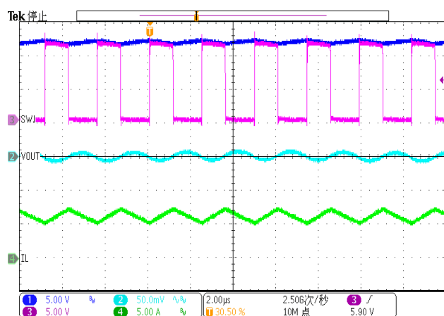
Figure 20. Output Ripple (Iload=6A)
