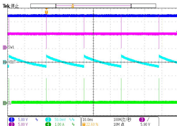
Figure 17. Output Ripple (Iload=0A, PFM)
