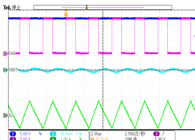
Figure 19. Output Ripple (Iload=0A, FPWM)
