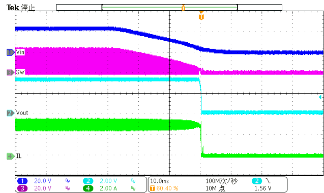
Figure 13. Power down(Iload=3A)
