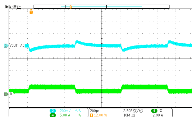
Figure 19. Load Transient (0.875A-2.625A, 1.6A/us)
