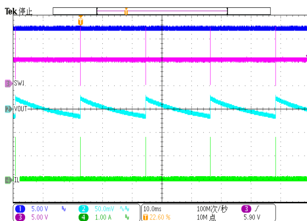
Figure 18. Output Ripple (Iload=0A, PFM)
