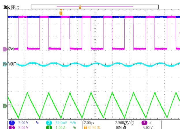
Figure 20. Output Ripple (Iload=0A, FPWM)
