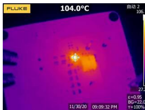
Figure 2. Thermal, 12VIN, Buck Iload=6A, LDO Iload=0.1A
