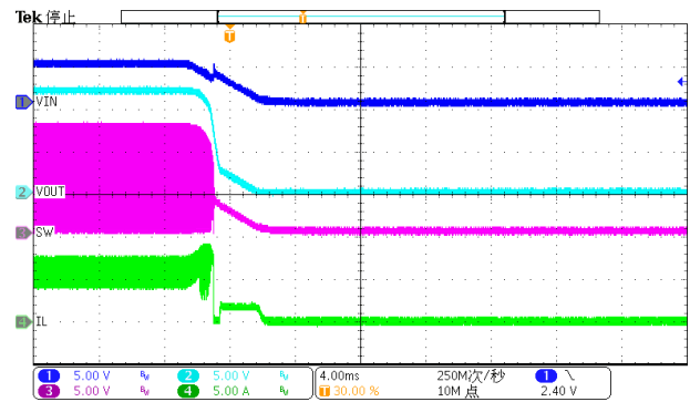
Figure 24. Power down( I_{load}=2A )
