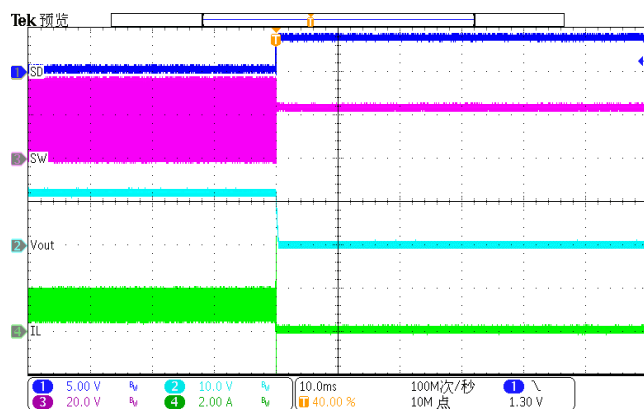
Figure 33. Shutdown entry
