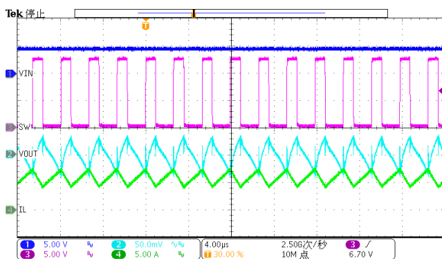
Figure 27. Steady-state ( I_{load}=2A )
