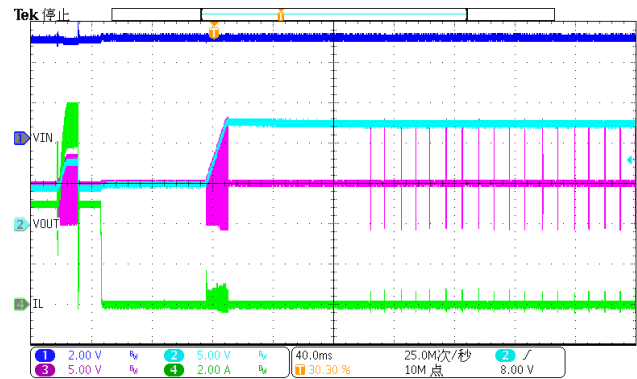
Figure 26. Over current recovery ( I_{load}=5A )
