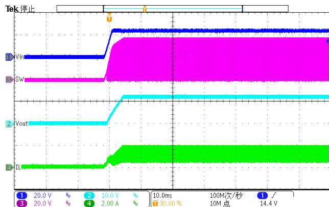
Figure 31. Power up(Iload=2A)
