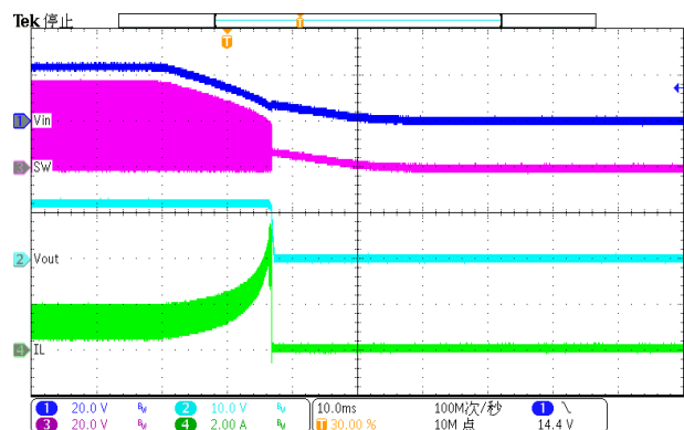
Figure 32. Power down(Iload=2A)
