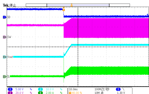
Figure 34. Shutdown remove
