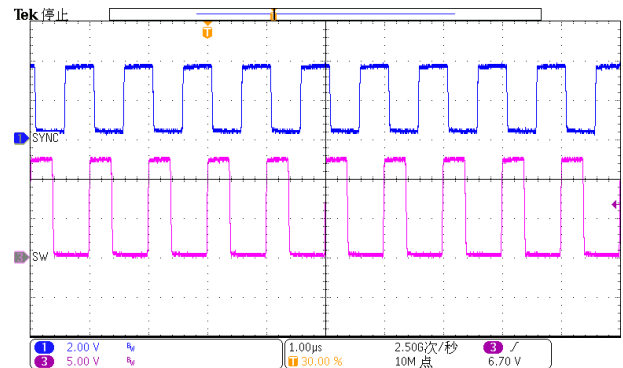
Figure 28. Sync Frequency
