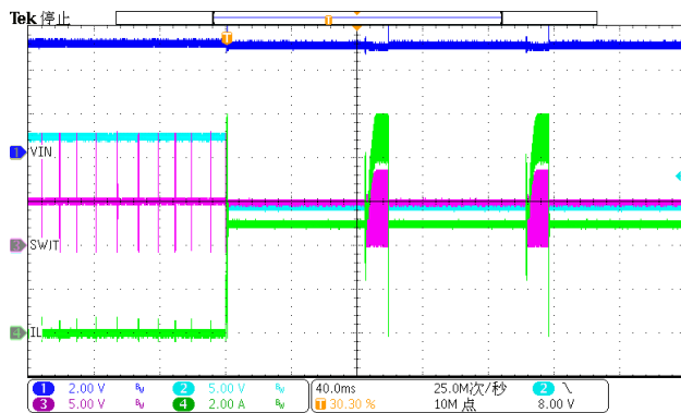
Figure 25. Over current protection ( I_{load}=5A )
