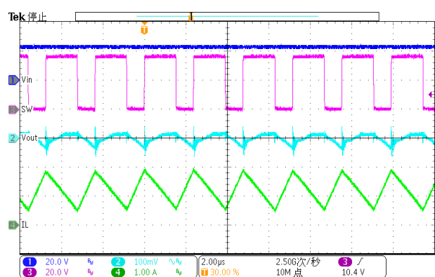
Figure 36. steady-state (Iload=2A)
