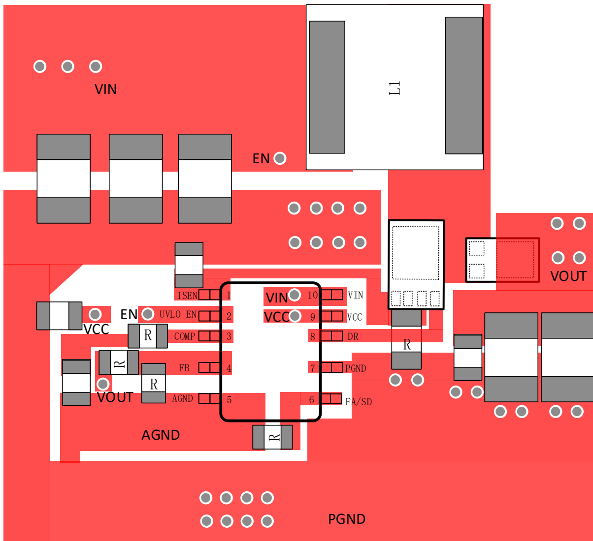
Figure 37. BOOST PCB Layout
